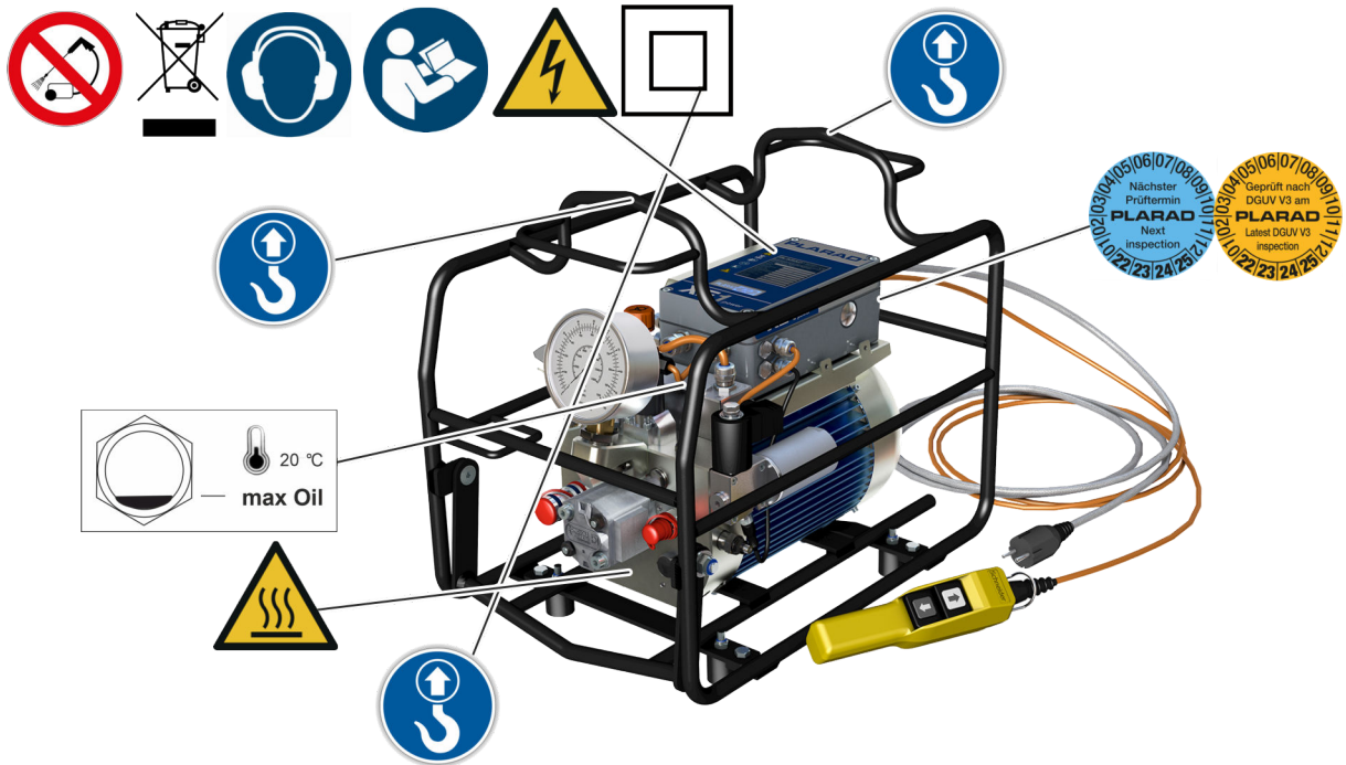
Fig. 14: Symbols on the hydraulic power pack
