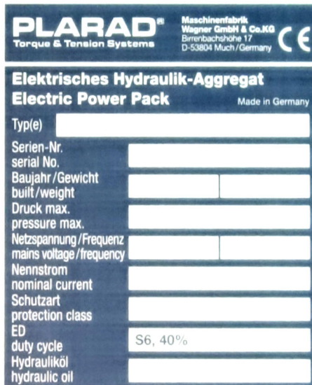
Fig. 6: Rating plate
