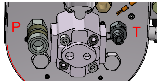
P (High pressure), T (Tank)
