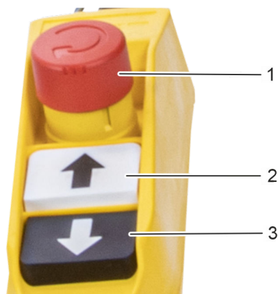
Fig. 8: Remote control without display
