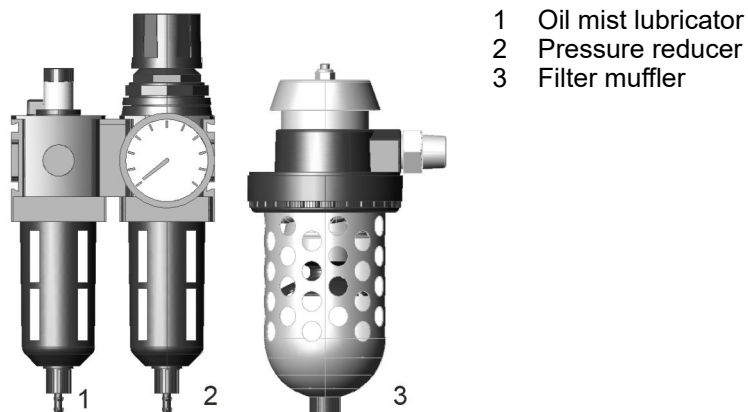
Fig. 7: Compressed air service unit
