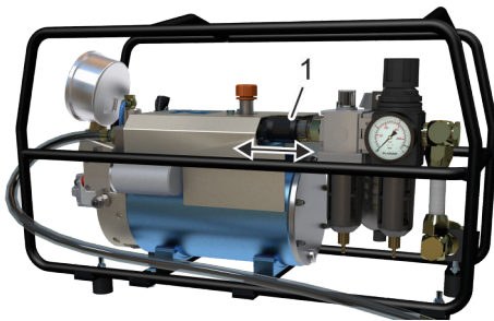
Fig. 25: Slide valve
